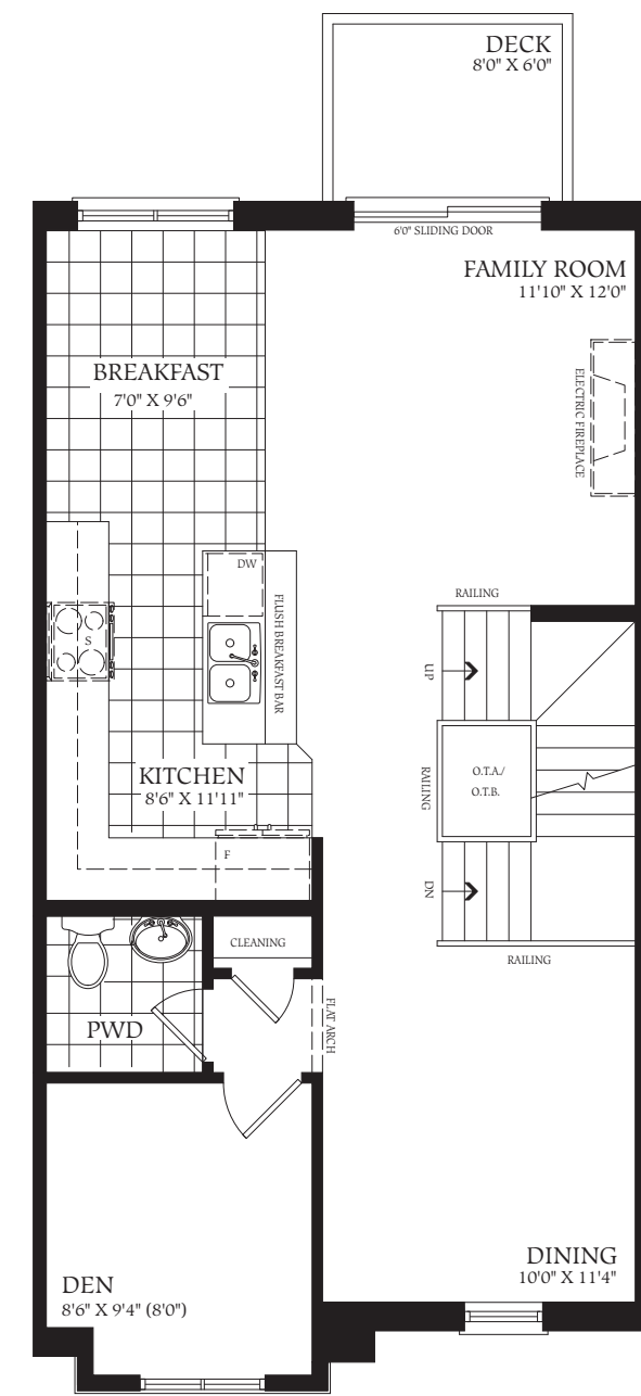
MAIN LEVEL 'A'
