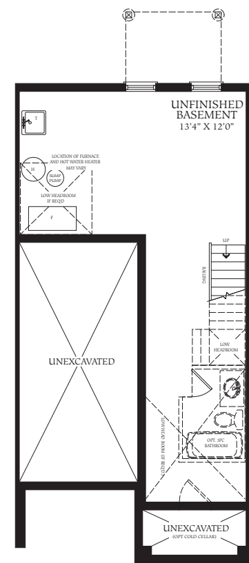
BASEMENT 'A'
