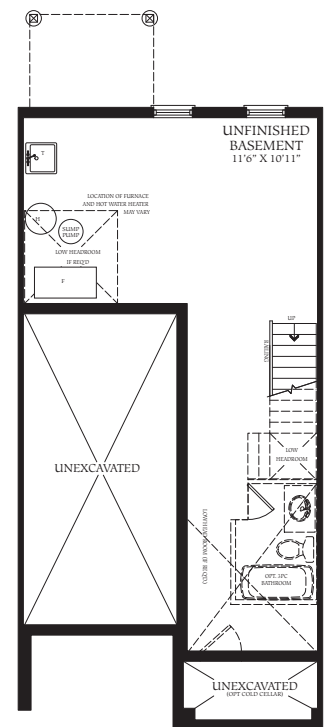
BASEMENT 'A'
