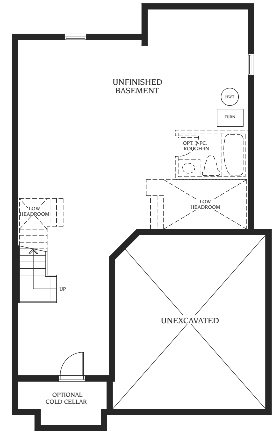
BASEMENT STYLE 'A'
