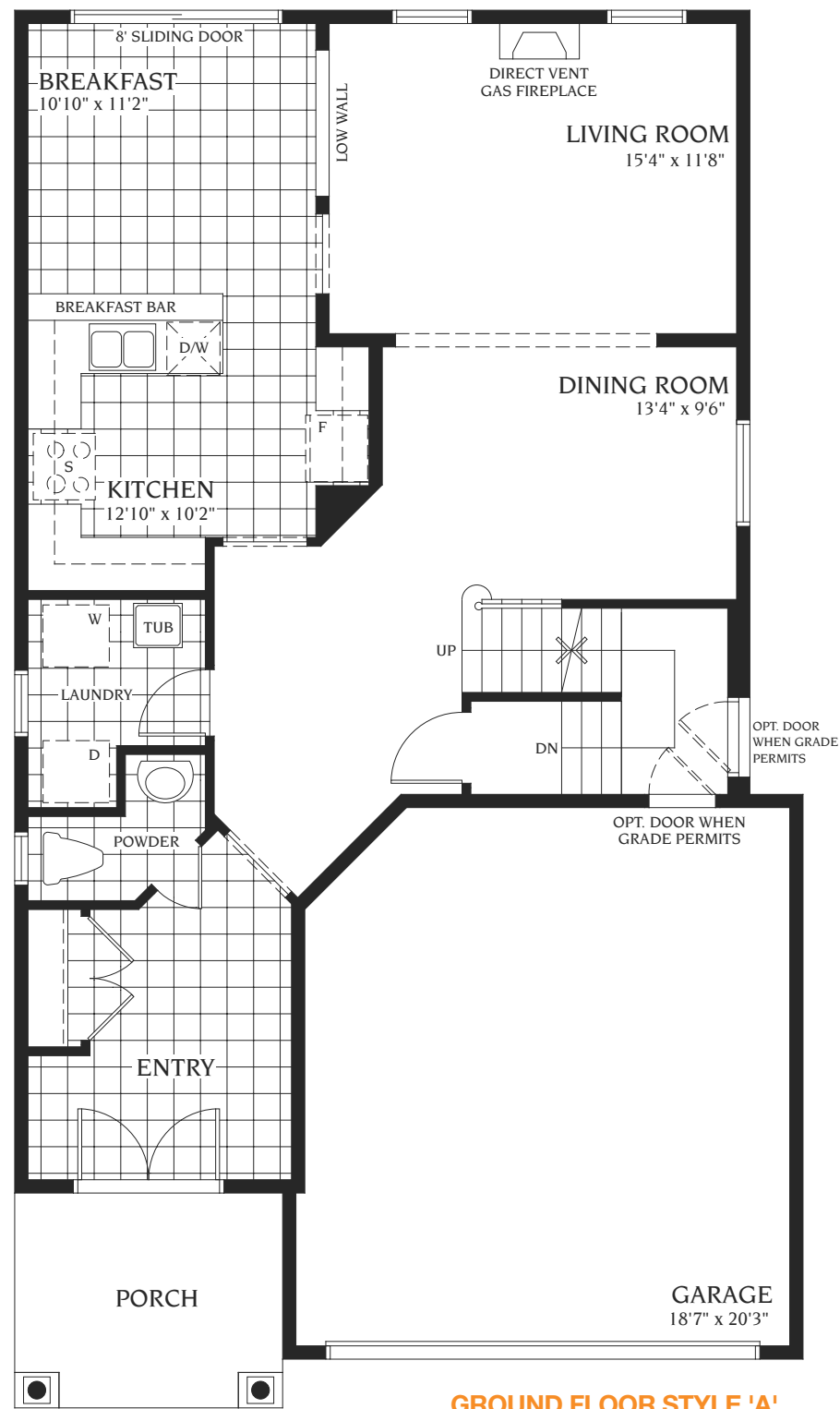
GROUND FLOOR STYLE 'A'
