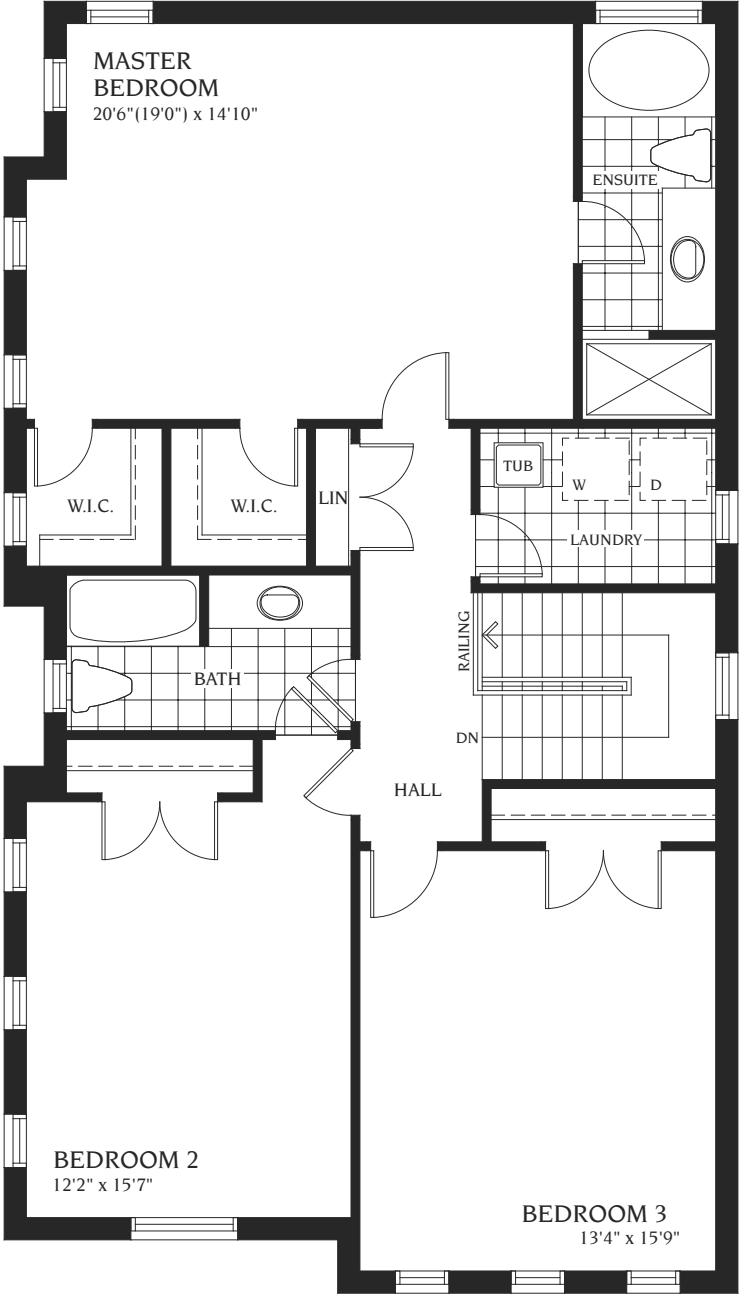
SECOND FLOOR STYLE 'B' 3 BEDROOM 2 BATH
