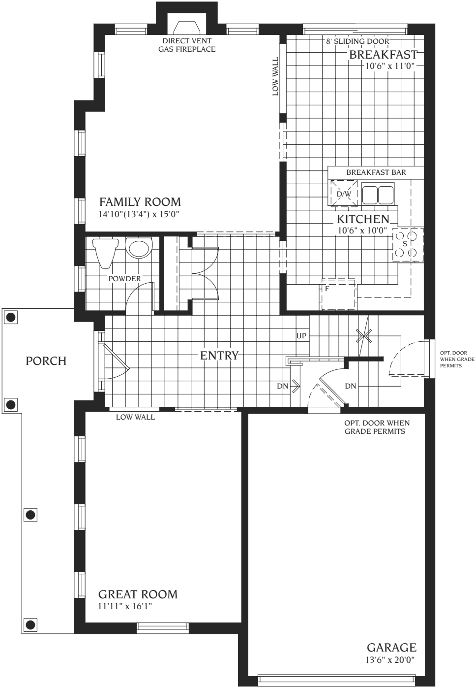
GROUND FLOOR STYLE 'B'
