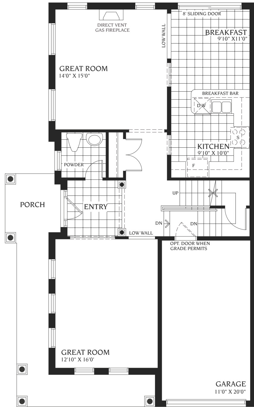
GROUND FLOOR STYLE 'B'
