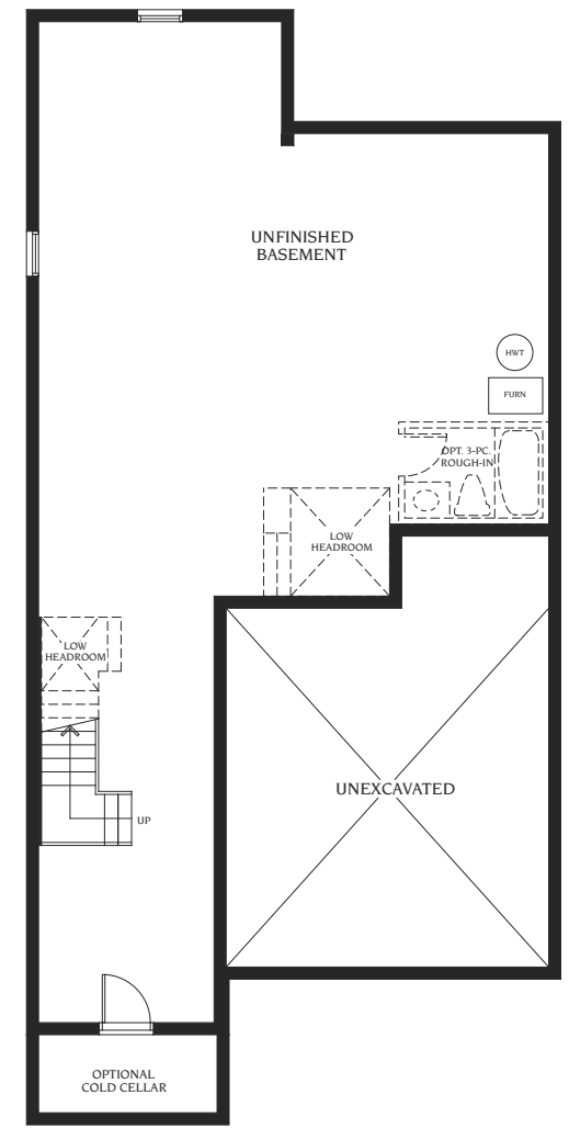
BASEMENT STYLE 'A'
